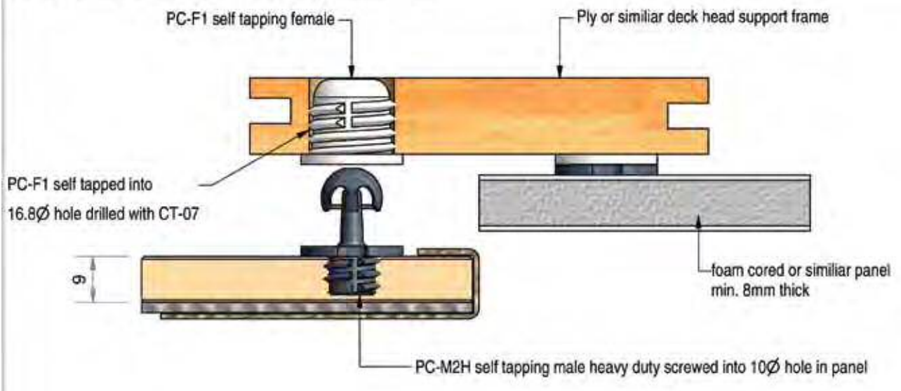
Partially exploded section through showing typical installation
